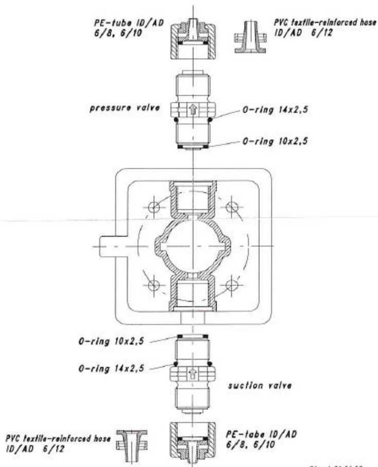
Installation drawing for suction and pressure valve EMP KKS
