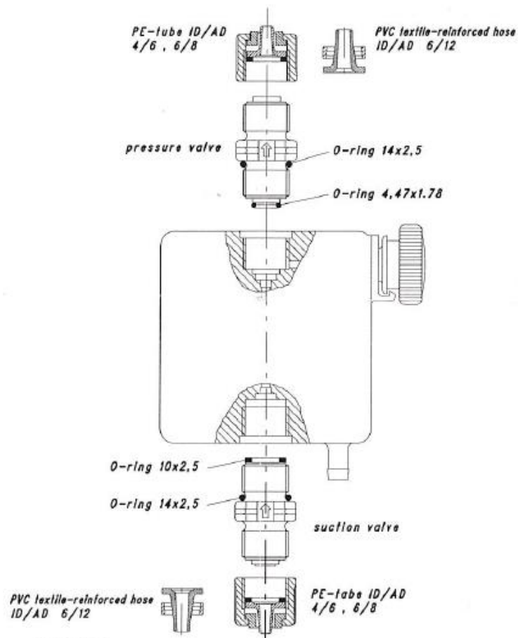
Installation drawing for suction and pressure valve EMP II
